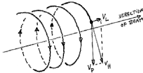
A Helical Particle Wave
