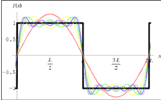
Fourier approximation of a Square into an infinite series of sine waves
